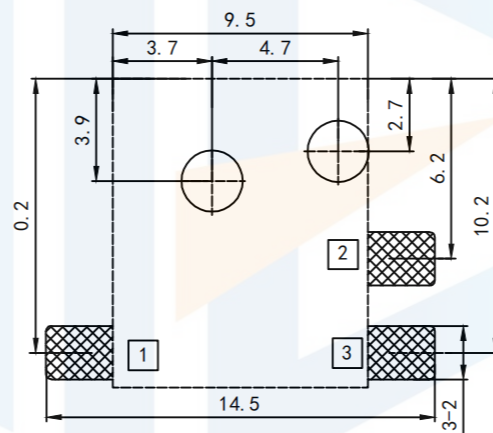
RECOMMENDED P. C. B LAYOUT UNSPECIFIED TOLERANCE: \pm 0.05 (BOTTOM VIEW)
