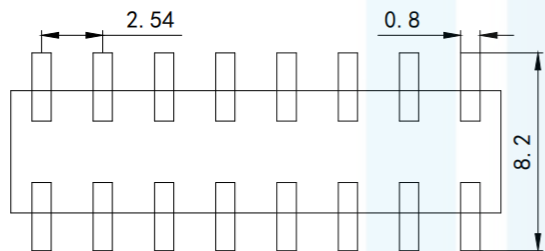
Recommended P.C.B Layout ( \pm 0.05 )
